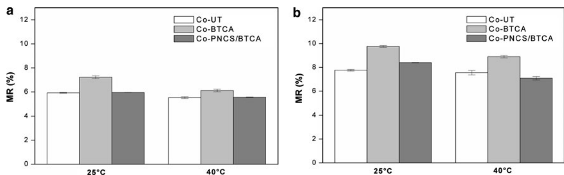
Fig. 5 Moisture regain (%) of Co-UT, Co-BTCA and Co-PNCS/BTCA at 50% R.H. (a) and 80% R.H. (b)
