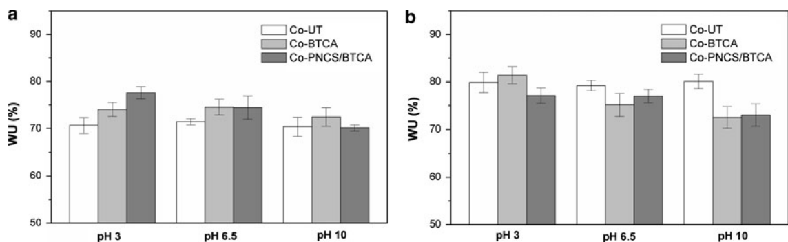
Fig. 1 Water uptake (WU) of Co-UT, Co-BTCA and Co-PNCS/BTCA at 25 °C (a) and 40 °C (b)
